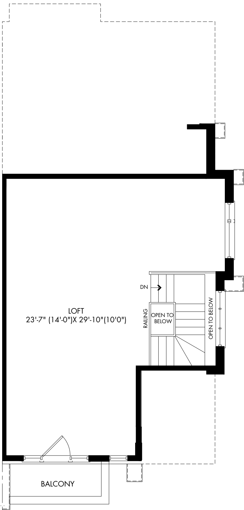
OPT. LOFT PLAN ELEV. A
