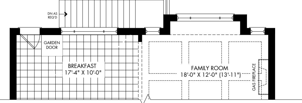
OPTIONAL GROUND FLOOR WITH EXTERIOR STAIRS ELEV. A
