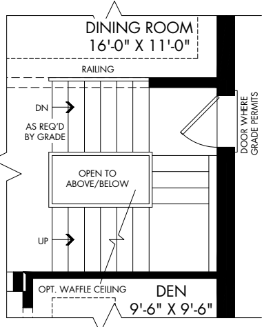
OPTIONAL GROUND FLOOR WITH EXTERIOR STAIRS ELEV. A
