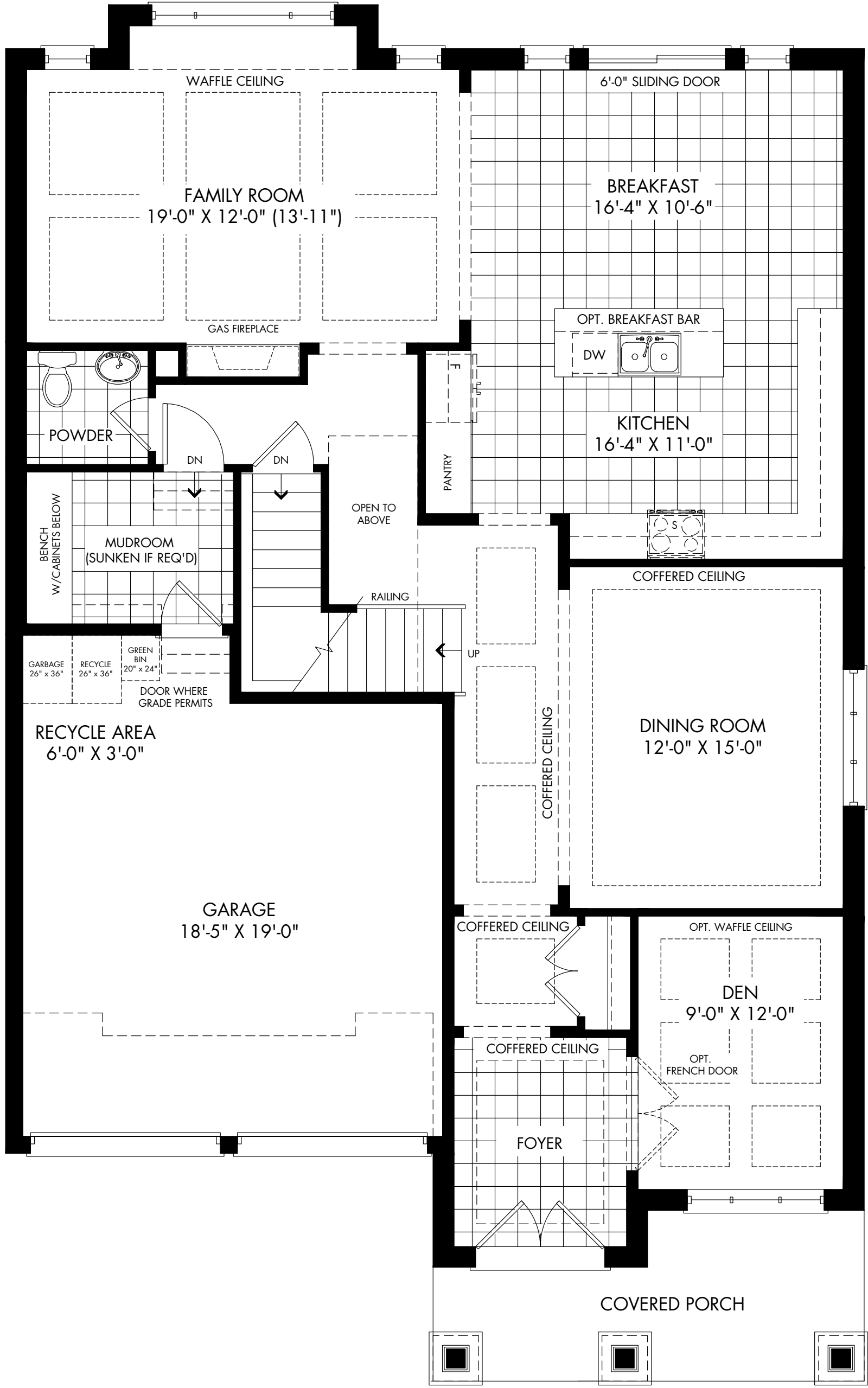
GROUND FLOOR ELEV. A
