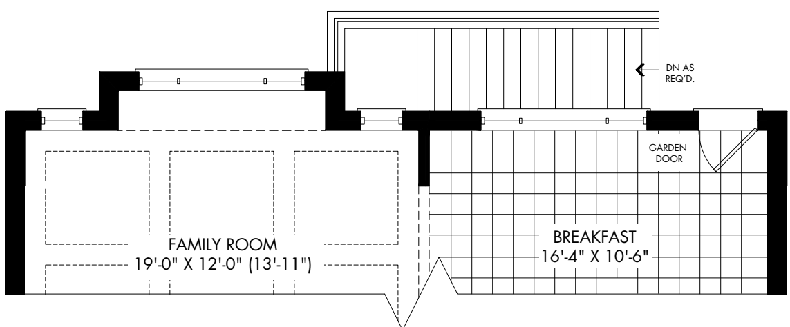
OPTIONAL GROUND FLOOR WITH EXTERIOR STAIRS ELEV. A, B & C
