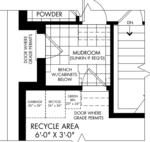
OPTIONAL GROUND FLOOR WITH EXTERIOR STAIRS ELEV. A, B & C
