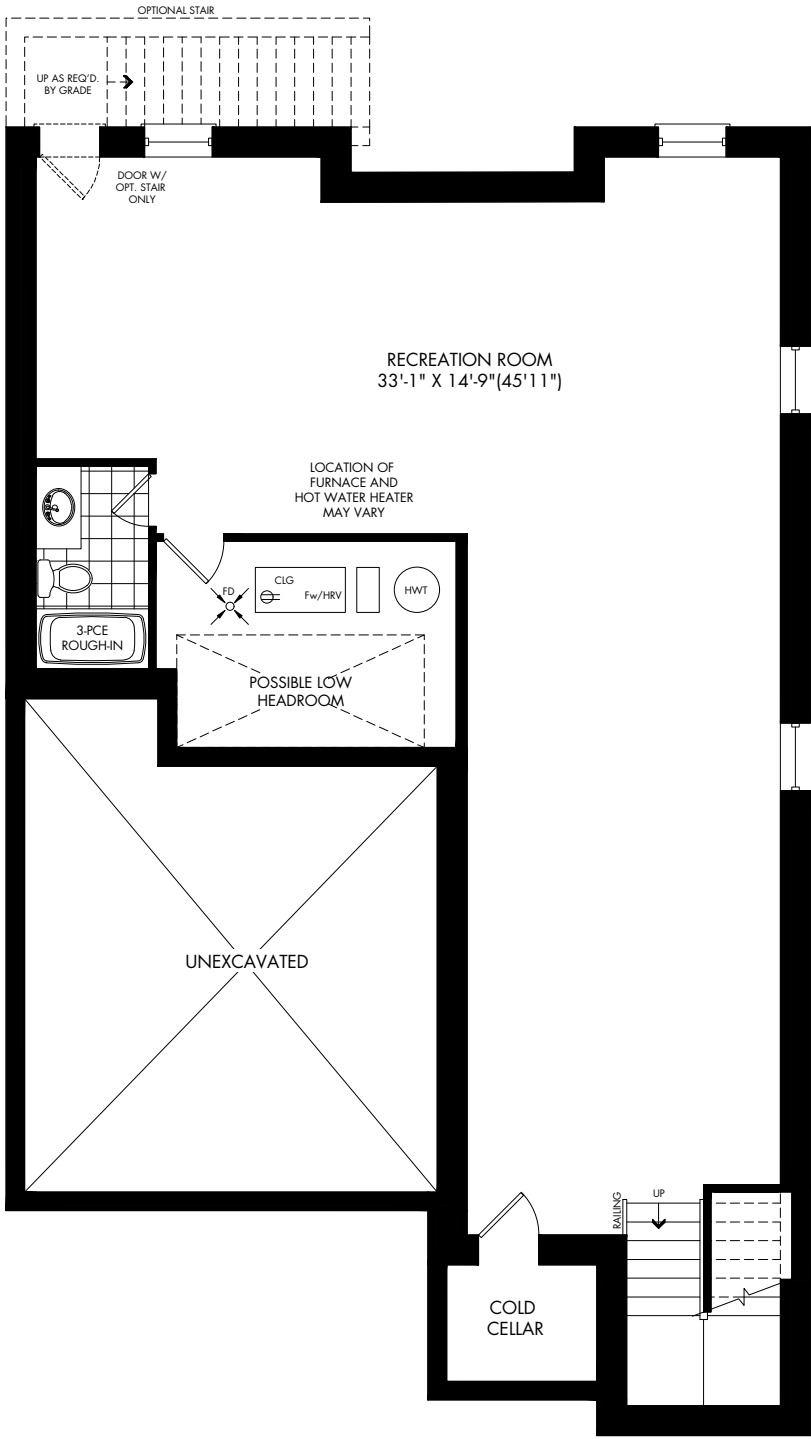
FINISHED BASEMENT ELEV. A & B
