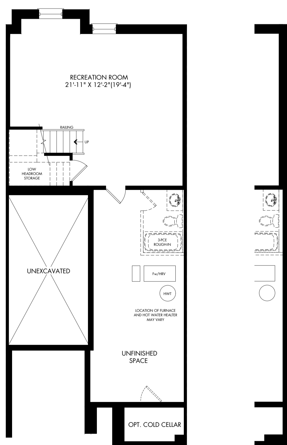
PART. FINISHED BASEMENT END ELEV. A
