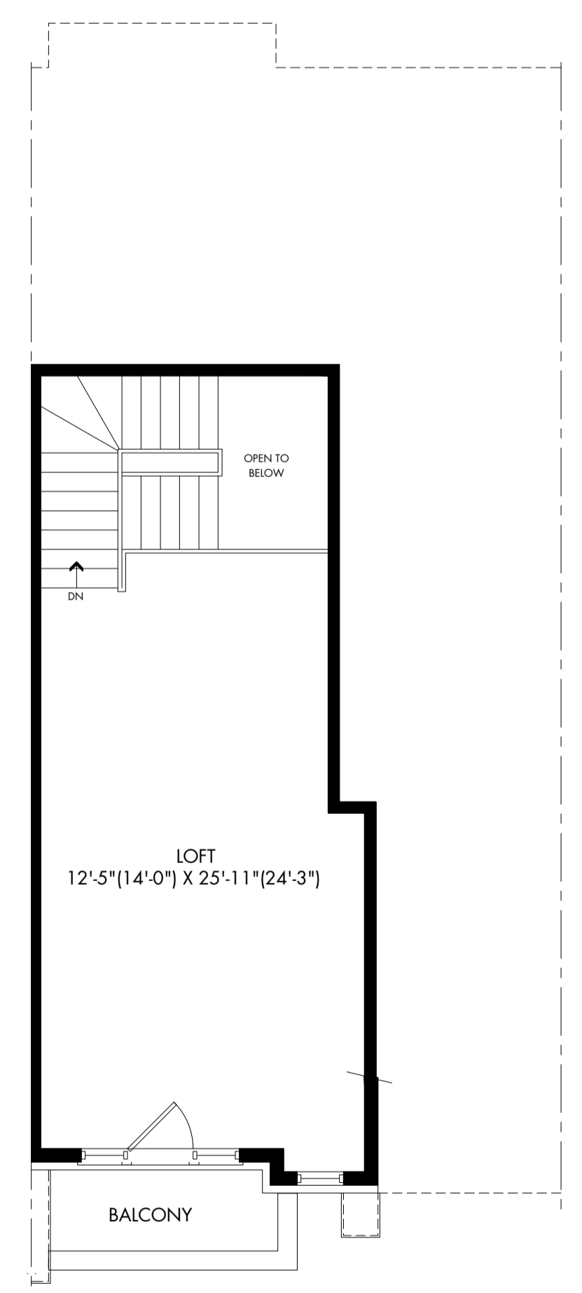
OPT. LOFT PLAN ELEV. A
