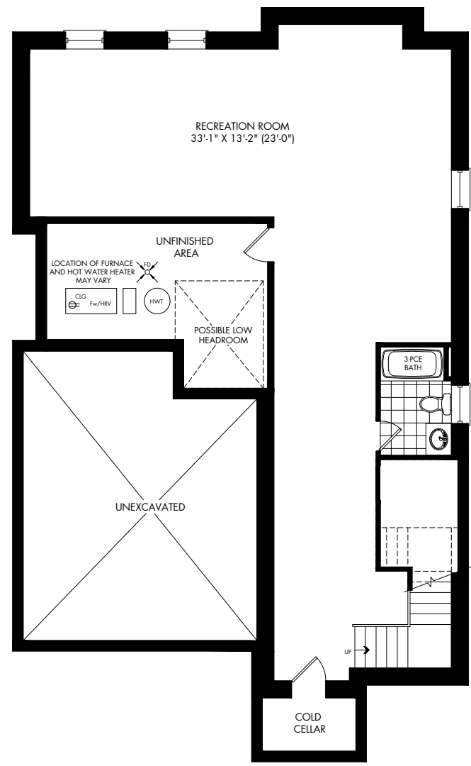
FINISHED BASEMENT ELEV. A, B & C
