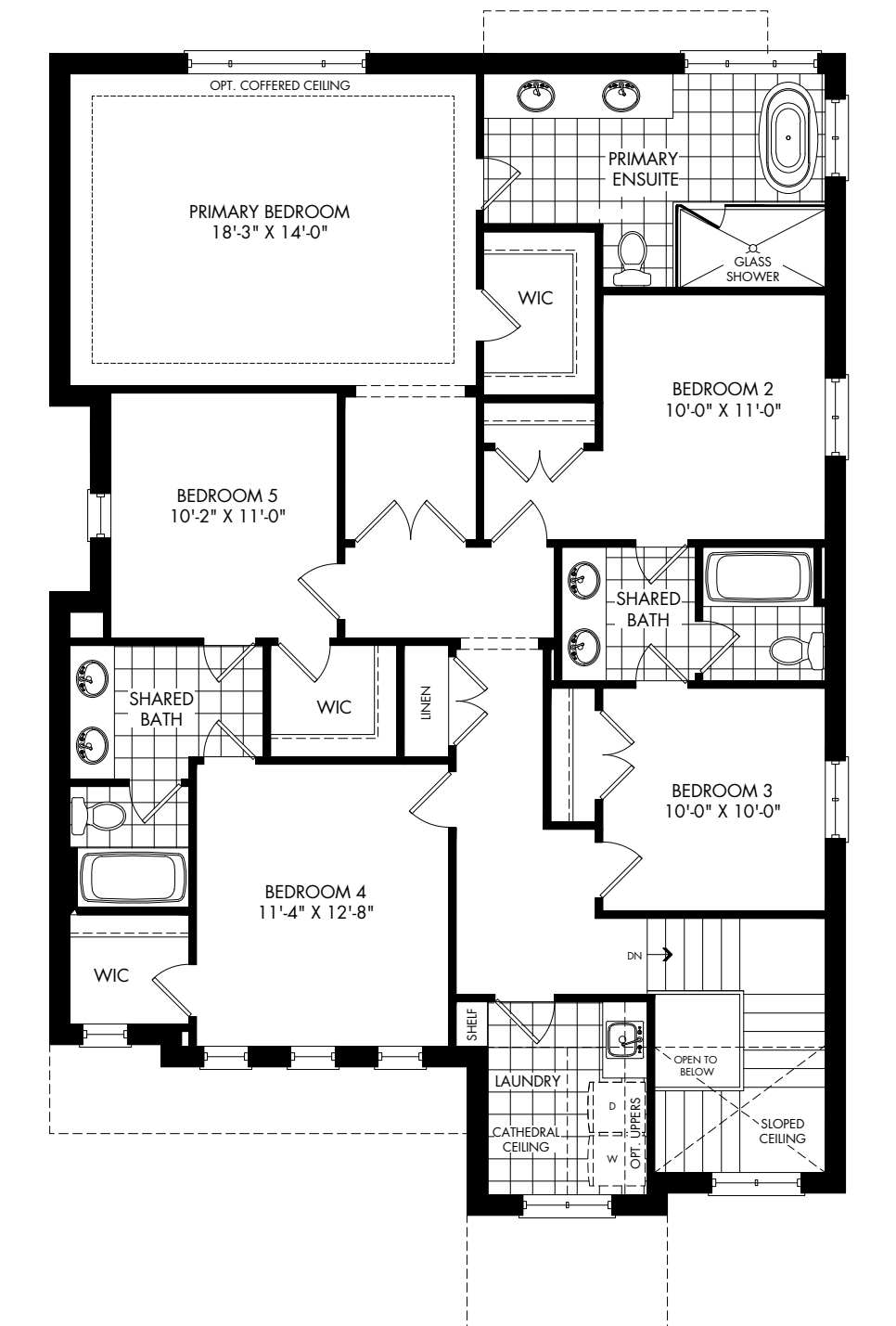
OPTIONAL SECOND FLOOR ELEV. A 5 BEDROOM
